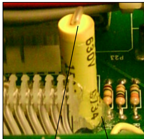
A close-up shows the cap installed on end due to a lack of room. NOTE: heat shrink tubing & RTV silicone.
