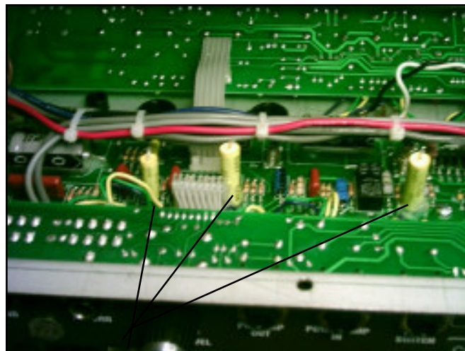
An additional view of the Fender® SuperSonic shows the Mallory® type 150M Series - metalized polyester film caps.
