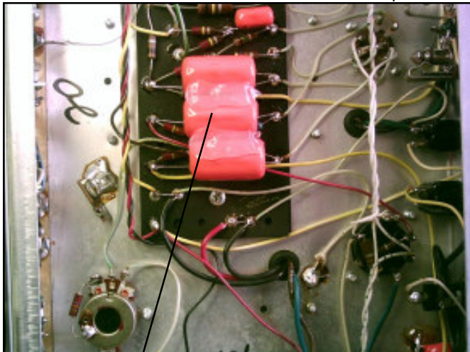
Cap upgrade in Fender® Super Reverb (Orange Drop - 716P Polypropylene Film caps with copper leads).
